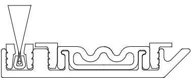
SECTION VIEW: ASSEMBLED RAIL, BRUSH, SEAL, RETAINERS.
