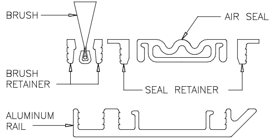
SECTION VIEW: EXPLODED RAIL, BRUSH, SEAL, RETAINERS.
