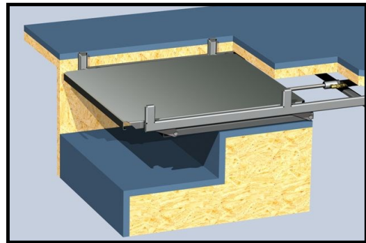
Intermediate Position
