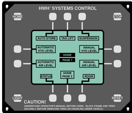
Standard Control Module Black & White (7W x 6H x 2.5D)
